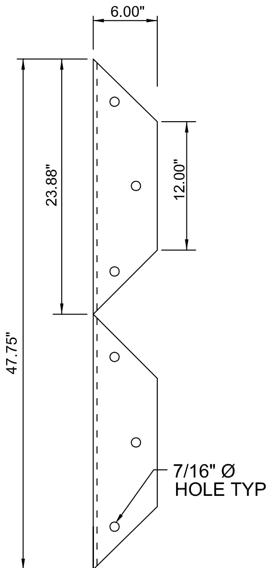
END VIEW
