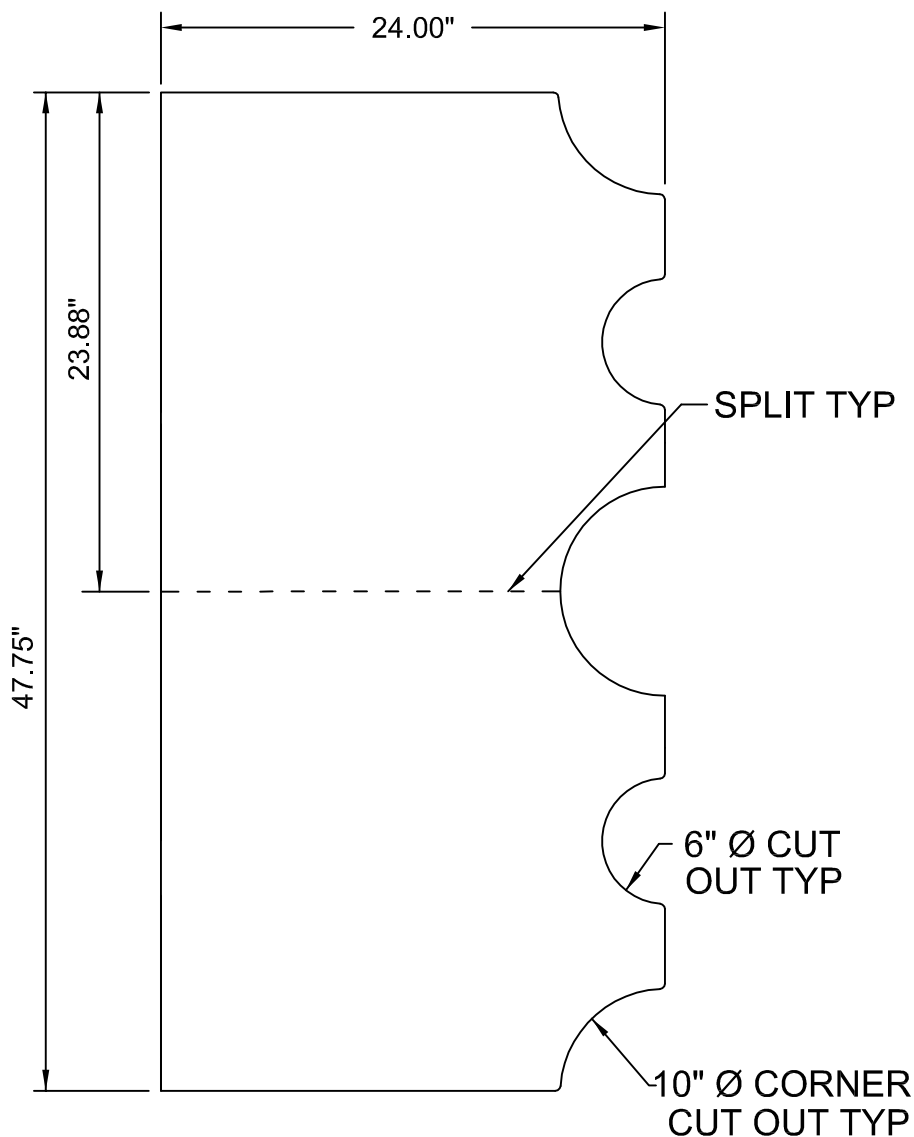
SIDE VIEW
